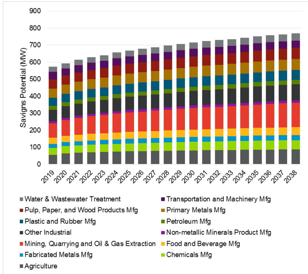
Figure D-8. Industrial Electric Demand Technical Potential by Customer Segment (MW)
