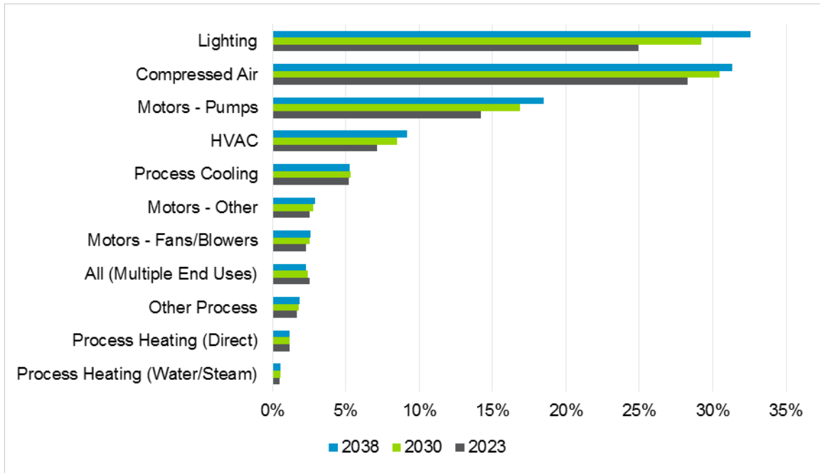
Figure 5-14. Industrial Electric Energy Technical Potential by End Use as a Percentage of End Use Forecast Consumption
