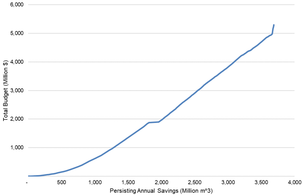
Figure F-46. Natural Gas Energy Cost Curve, Scenario C in 2038
