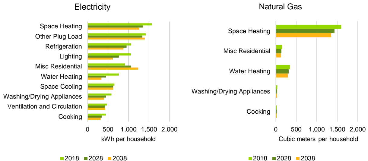
Figure B-2. Residential Energy Intensity by End Use (Electricity and Natural Gas)
