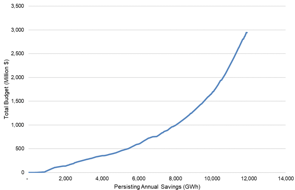
Figure F-23. Electric Energy Cost Curve, Scenario A in 2030
