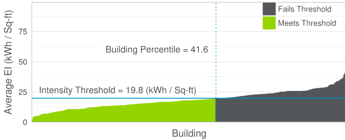
Figure G-7. Scenario A Potential Benchmarking – Electricity
