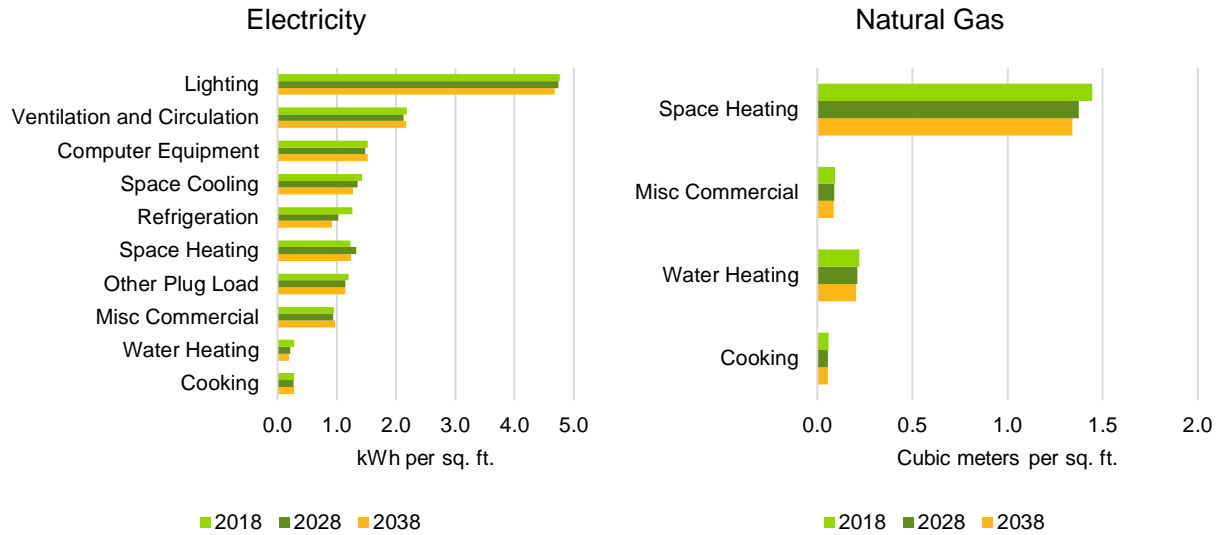
Figure B-6. Commercial Energy Intensity by End Use (Natural Gas and Electricity)
