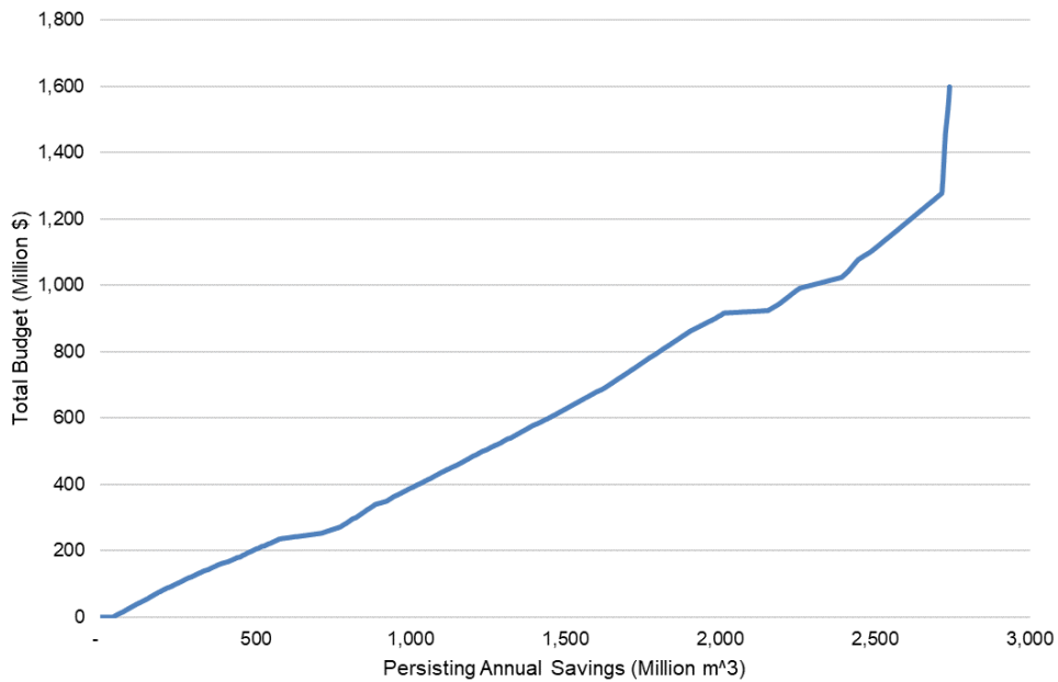
Figure F-28. Natural Gas Energy Cost Curve, Scenario A in 2038
