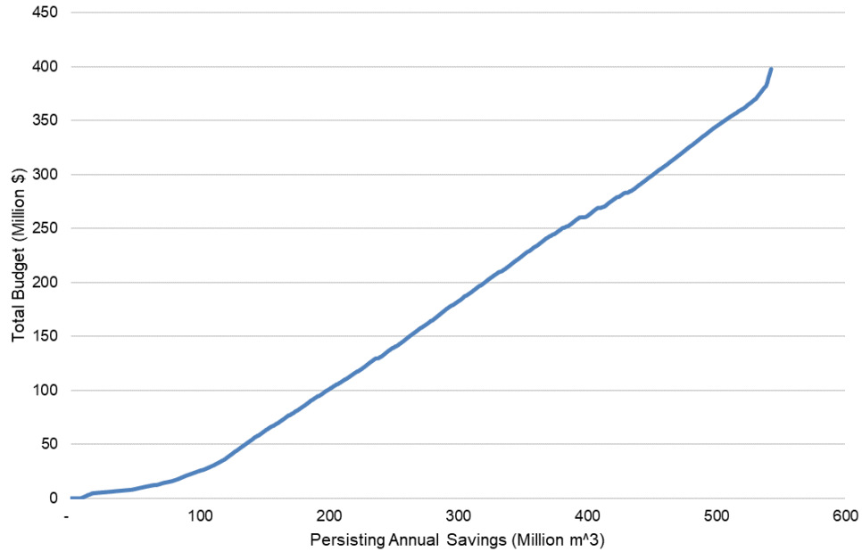
Figure F-22. Natural Gas Energy Cost Curve, Scenario A in 2023
