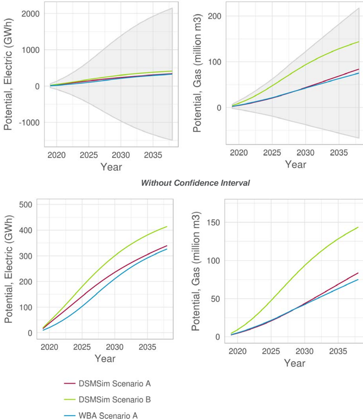
Figure 8-5. Enhanced Model Forecast Conservation Potential – 2019-2038
