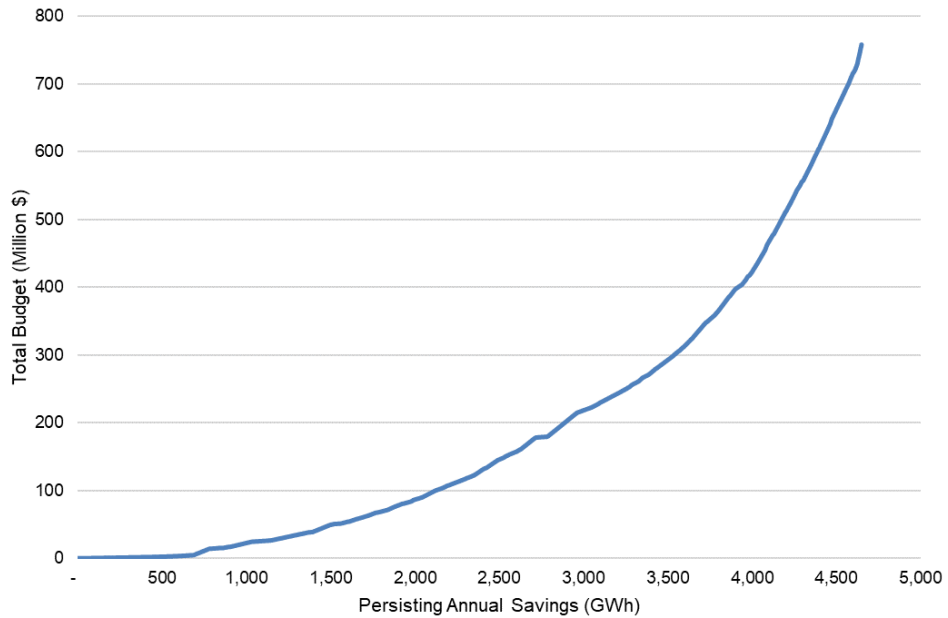
Figure F-47. Electric Energy Cost Curve, Scenario D in 2023
